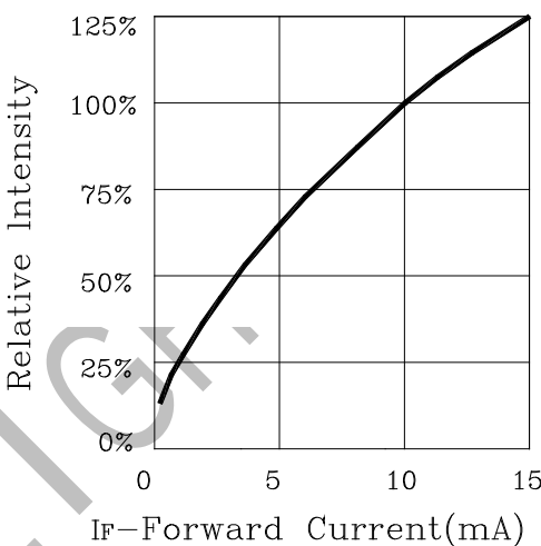
RELATIVE INTENSITY Vs. FORWARD CURRENT
