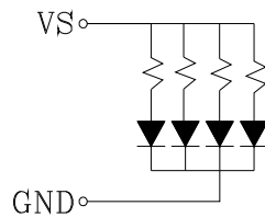
Recommended Set-up
