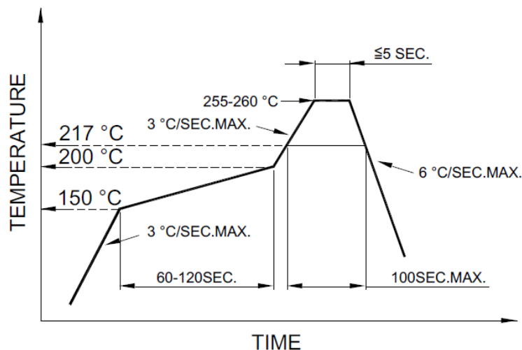
Pb free reflow soldering Profile
