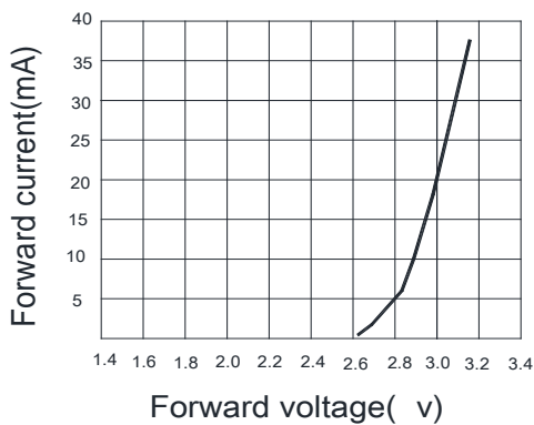
Voltage current relationship
