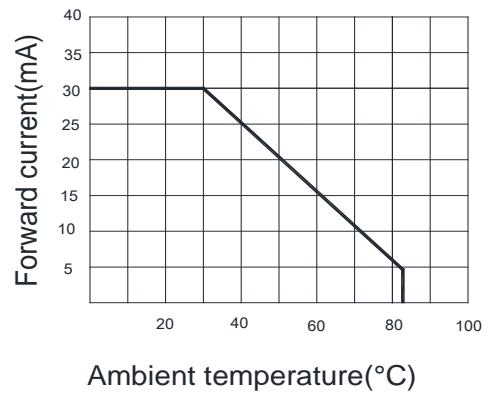
Current and ambient temperature
