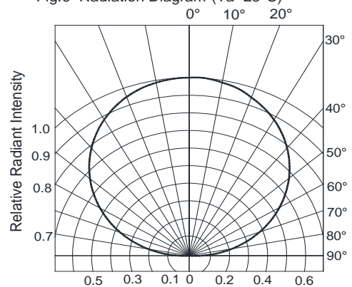
Fig.6 Radiation Diagram ( T_a=25^{\circ}\text{C} )
