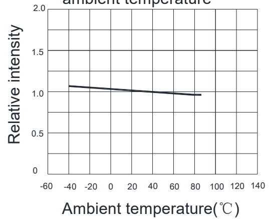
Relative light intensity vs ambient temperature
