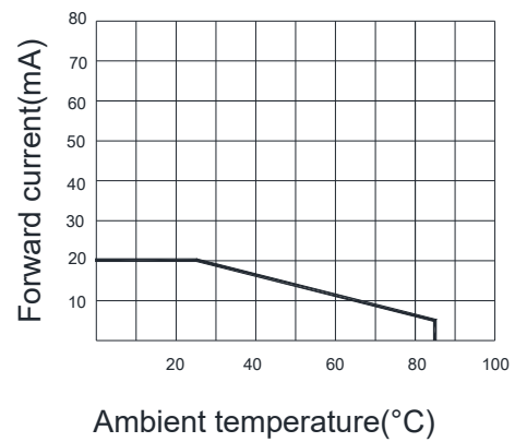
Current and ambient temperature
