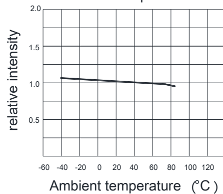
Relative light intensity vs ambient temperature
