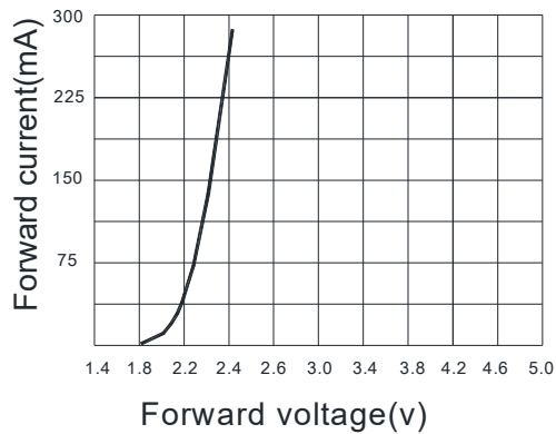
Voltage current relationship
