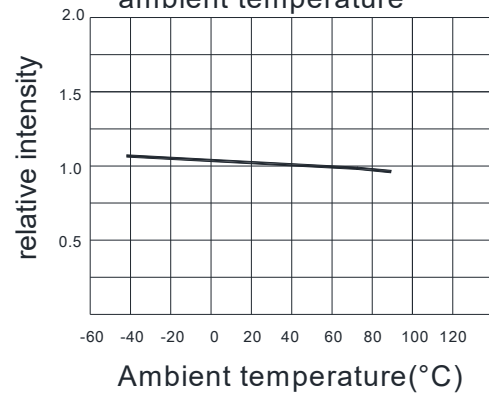
Relative light intensity vs ambient temperature
