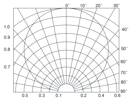
Radiation angle
