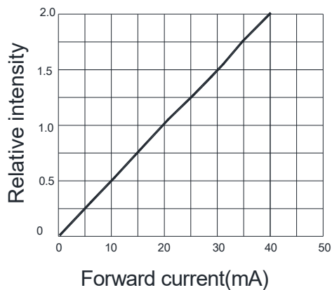
Relative light intensity vs current
