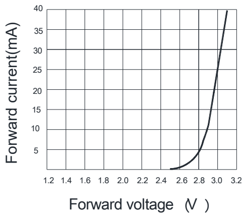
Voltage current relationship
