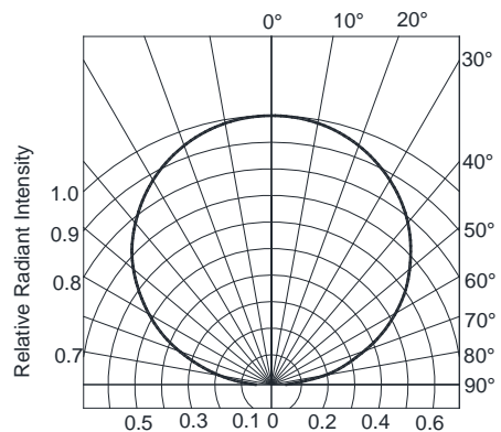
Fig.6 Radiation Diagram (Ta=25°C)
