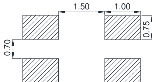
Recommended solder pad
