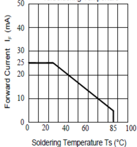
Fig.5-Max. Driving Forward Current vs. Soldering Temperature
