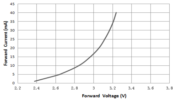
Forward Current VS. Forward Voltage (Ta=25°C)
