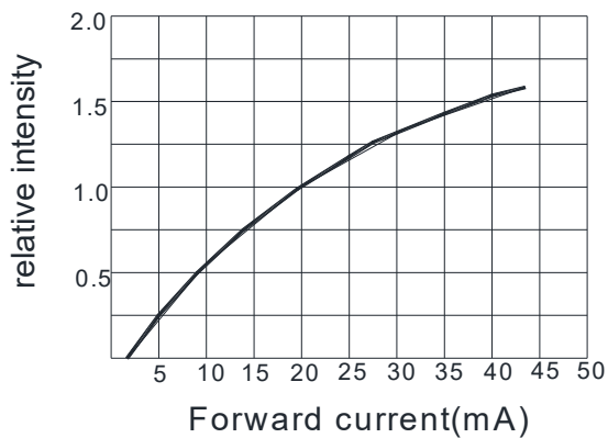
Relative light intensity vs current
