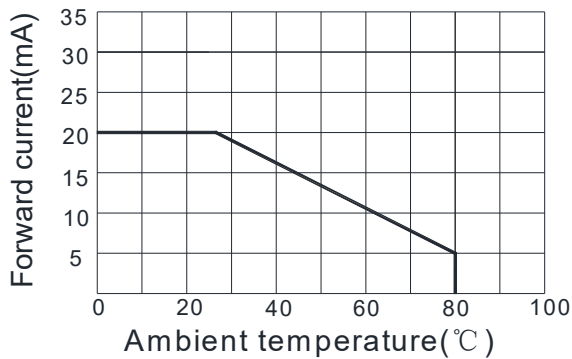
Current and a`mbient temperature
