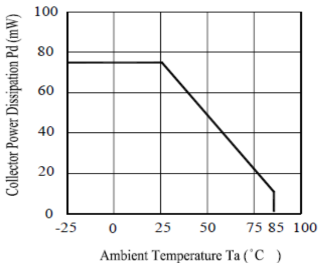
Fig.1 Collector Power Dissipation vs. Ambient Temperature
