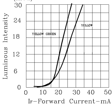
Luminous Intensity VS. (mcd) Forward Current
