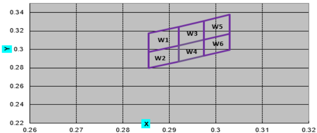
C.I.E.Chromaticity Diagram
