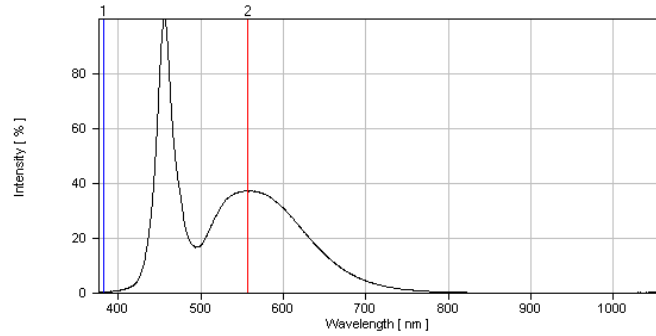
Fig.1 White Relative Intensity vs. Wavelength
