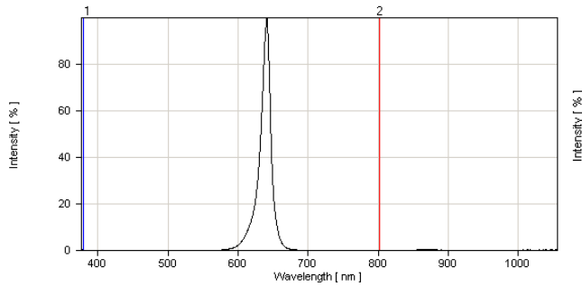
Fig.1 Red Relative Intensity vs. Wavelength
