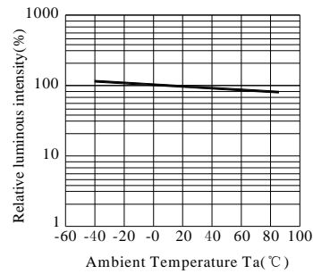
Fig.5 Luminous Intensity vs.Ambient Temperature
