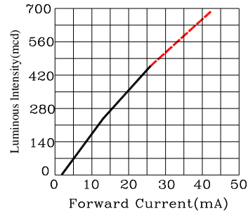
Fig.3 Luminous Intensity vs.Forward Current
