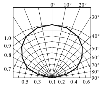
Fig.7 Relative Intensity vs.Angle
