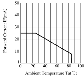
Fig.6 Forward Current Derating Curve
