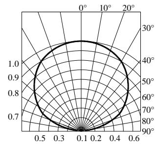
Fig.7 Relative Intensity vs.Angle
