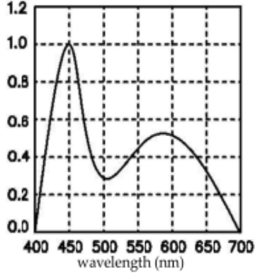
Spectral Distribution Relative Intensity VS. Wavelength (Ta=25°C)
