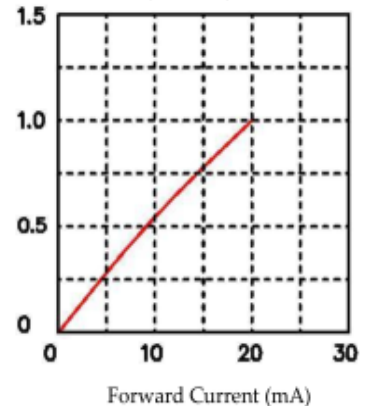
Relative Intensity VS. Forward Current (Ta=25°C)
