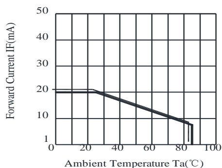
Fig.6 Forward Current Derating Curve
