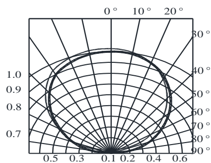
Fig.7 Relative Intensity vs. Angle
