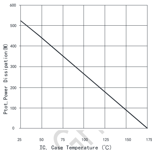
Fig. 2 Power dissipation vs. case temperature (Tvj≤175°C)
