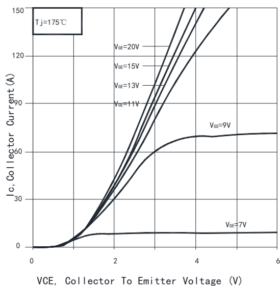
Fig. 5 Typical output characteristic ( T_j=175^{\circ}\text{C} )
