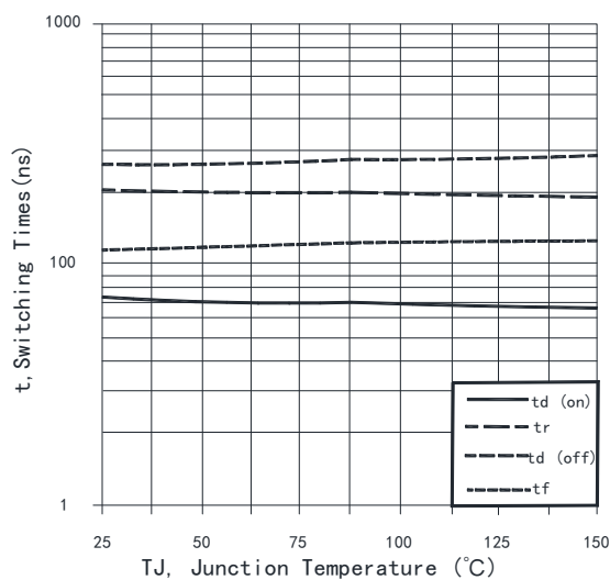
Fig. 10 Typical switching times vs. T_j (Ind. Load, V_{CE} = 400\text{V} , V_{GE} = 15/0\text{V} , I_C = 75\text{A} , R_g = 10\Omega )
