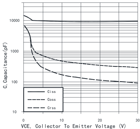
Fig. 12 Typical capacitance vs. collector-emitter voltage ( V_{GE} = 0\text{V} , f = 1\text{MHz} )
