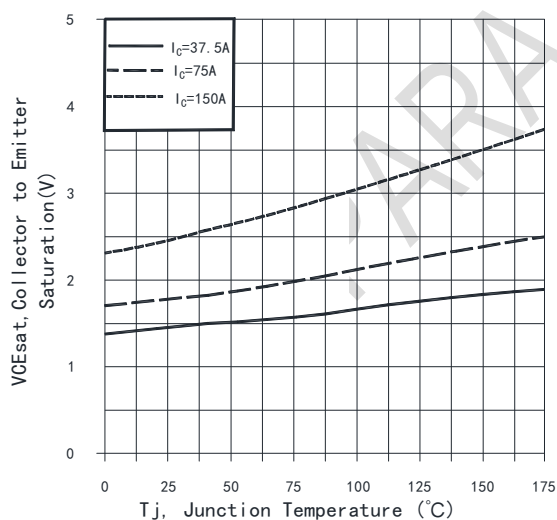
Fig. 7 Typical collector-emitter saturation voltage vs. T_j ( V_{GE}=20\text{V} )
