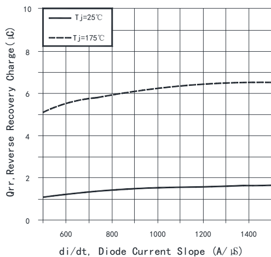
Fig. 17 Typical reverse recovery charge vs. diode current slope (VR=400V)
