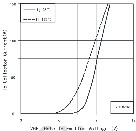
Fig. 6 Typical transfer characteristic ( V_{CE}=20\text{V} )
