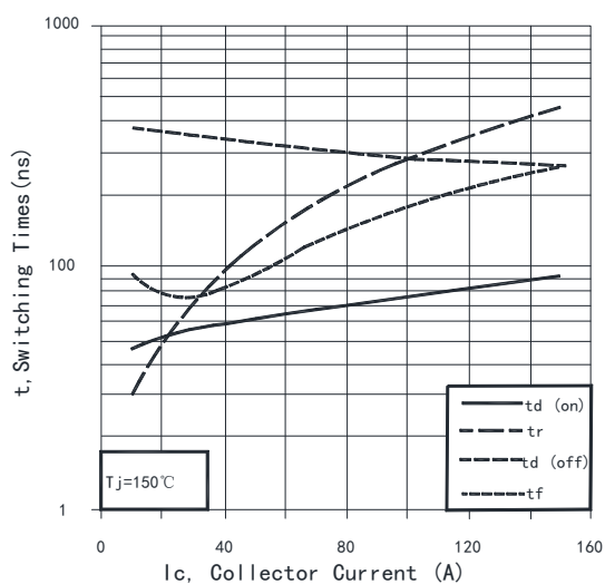
Fig. 8 Typical switching times vs. collector current (Ind. load, T_j=150^{\circ}\text{C} , V_{CE}=400\text{V} , V_{GE}=15/0\text{V} , R_g=12\Omega )
