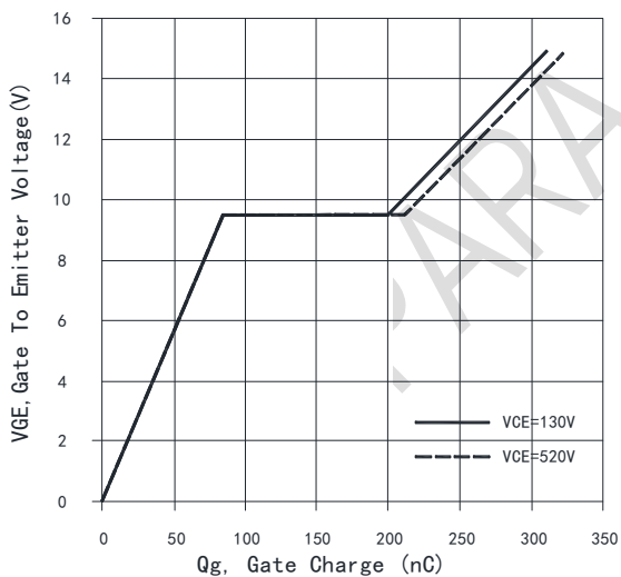
Fig. 11 Typical gate charge ( I_C = 75\text{A} )
