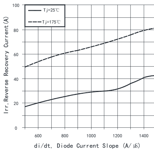
Fig. 18 Typical reverse recovery current vs. diode current slope (VR=400V)
