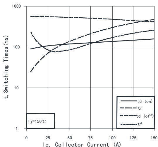
Fig. 9 Typical switching times vs. collector current ( T_j=150^\circ\text{C} , V_{CE}=600\text{V} , V_{GE}=15\text{V} , R_g=10\Omega )
