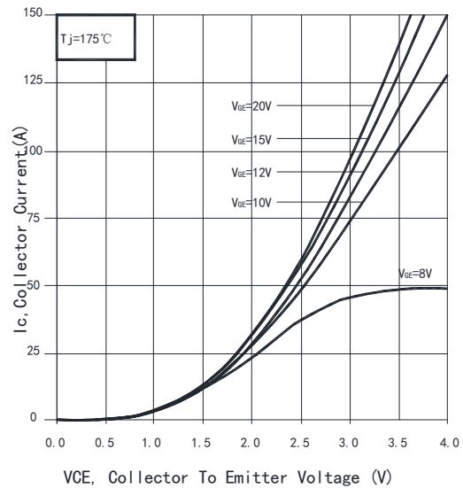
Fig. 4 Typical output characteristic ( T_{vj} = 175^{\circ}\text{C} )
