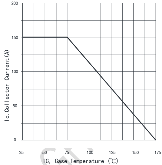
Fig. 2 DC Collector current vs. Case temperature ( V_{GE} \leq 15\text{V} , T_{vj} \leq 175^{\circ}\text{C} )
