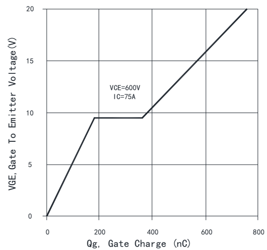
Fig. 8 Typical gate charge ( I_C=75A , V_{CE}=600V , T_{vj} = 25^\circ C )
