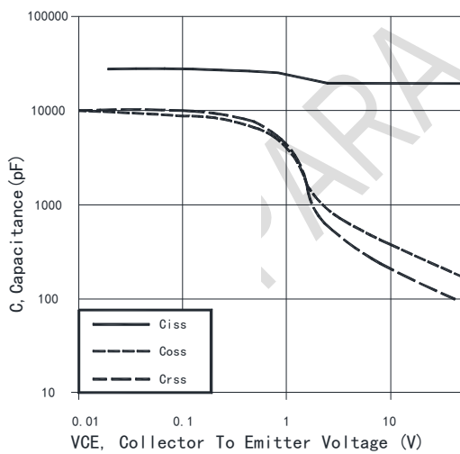
Fig. 7 Typical capacitance vs. collector-emitter voltage ( V_{GE}=0V , f=1MHz )
