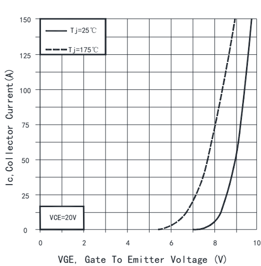
Fig. 5 Typical transfer characteristic ( V_{CE}=20V )
