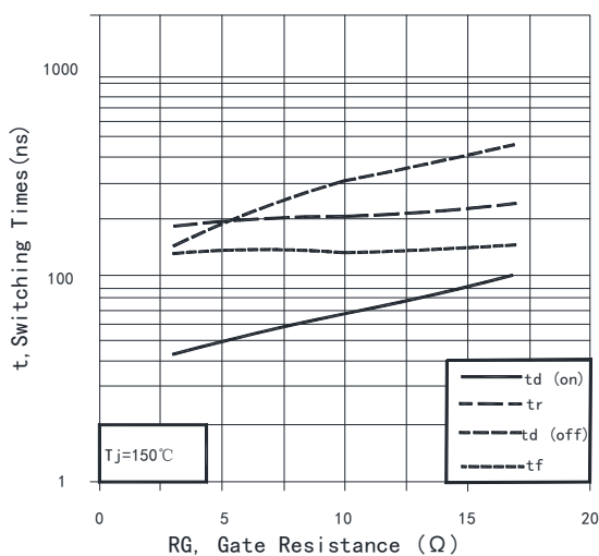
Fig. 9 Typical switching times vs. gate resistor (Ind. Load, T_{vj}=150^{\circ}\text{C} , V_{CE}=400\text{V} , V_{GE}=15/0\text{V} , I_C=75\text{A} )
