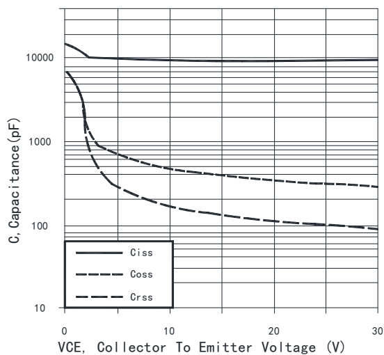
Fig. 12 Typical capacitance vs. collector-emitter voltage ( V_{GE}=0\text{V} , f=1\text{MHz} )
