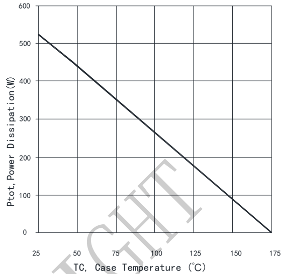
Fig. 2 Power dissipation vs. case temperature ( T_{vj}\leq 175^\circ\text{C} )
