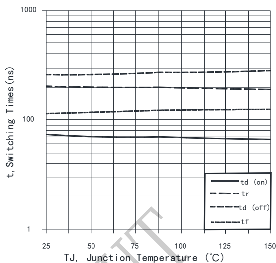
Fig. 10 Typical switching times vs. T_{vj} (Ind. Load, V_{CE}=400\text{V} , V_{GE}=15/0\text{V} , I_C=75\text{A} , R_g=10\Omega )
