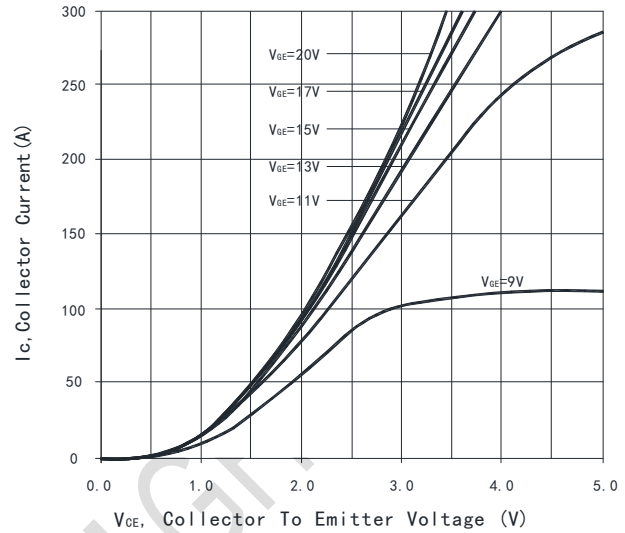
Fig. 2 Typical output characteristic ( T_{vj}= 150^\circ\text{C} )
