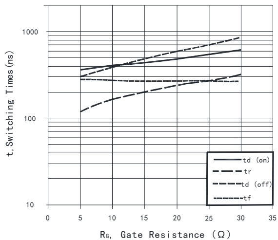
Fig. 4 Typical switching times vs. gate resistor (Ind. Load, T_{vj}= 150^\circ\text{C} , V_{CE}= 600\text{V} , V_{GE}= 15/0\text{V} , I_C= 150\text{A} )
