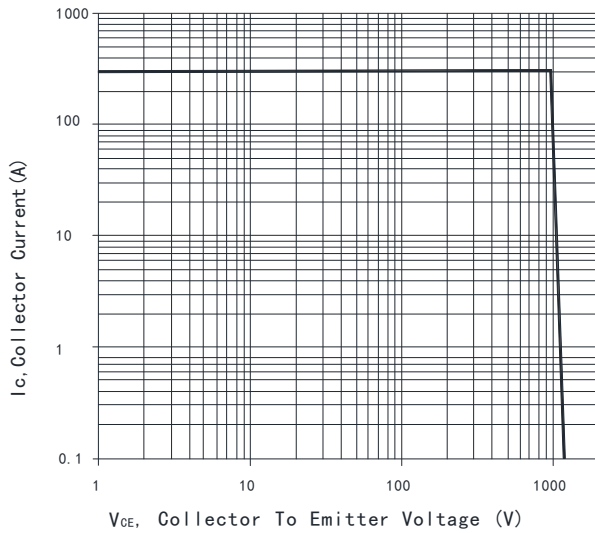
Fig. 1 Reverse bias safe operating area ( D= 0 , T_C= 25^\circ\text{C} , T_{vj}\leq 150^\circ\text{C} ; V_{GE}= 15\text{V} )
