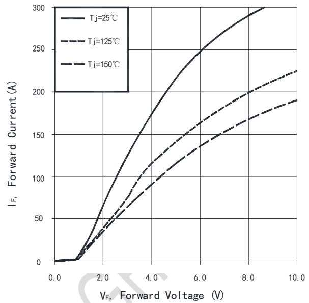
Fig. 6 Typical diode forward current vs. forward voltage
