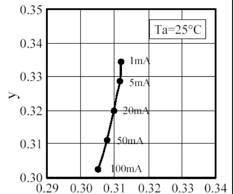
■ Forward Current vs. Chromaticity Coordinate
