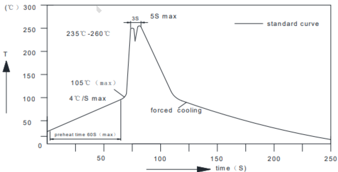
WAVE SOLDER PROFILE
