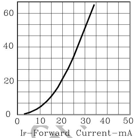
Luminous Intensity VS. Forward Current (cd)
