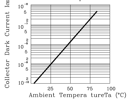
Fig. 2 Collector Dark Current I_{c0} (A) vs. Ambient Temperature
