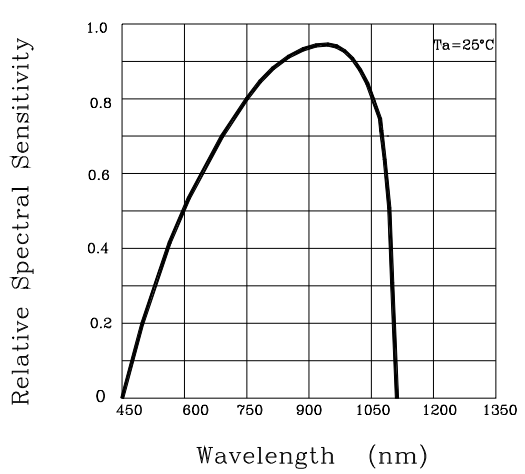
Fig. 5 Spectral Sensitivity
