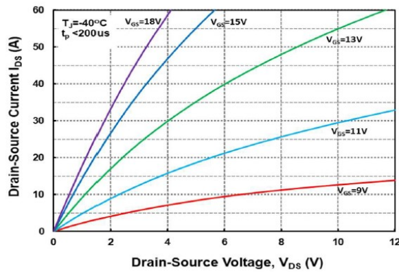
Figure 1. Output Characteristics, T_J = -40^\circ\text{C}
