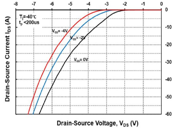
Figure 8. Body Diode Characteristics @ -40°C
