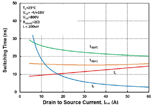
Figure 25. Switching Times vs Drain Current ( V_{DS}=800\text{V} )
