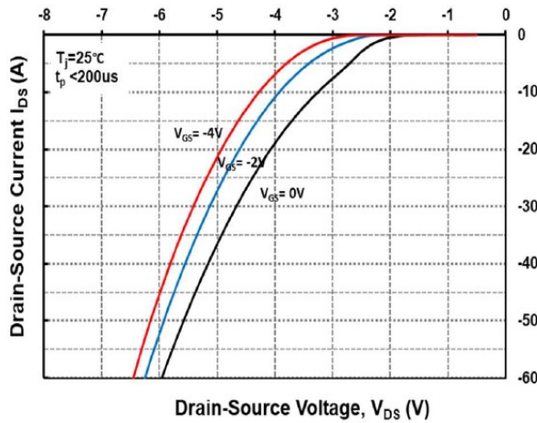
Figure 9. Body Diode Characteristics @ 25°C
