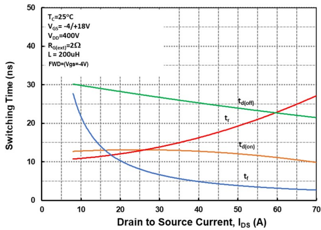
Figure 25: Switching Times vs Drain Current(V DD =400V)
